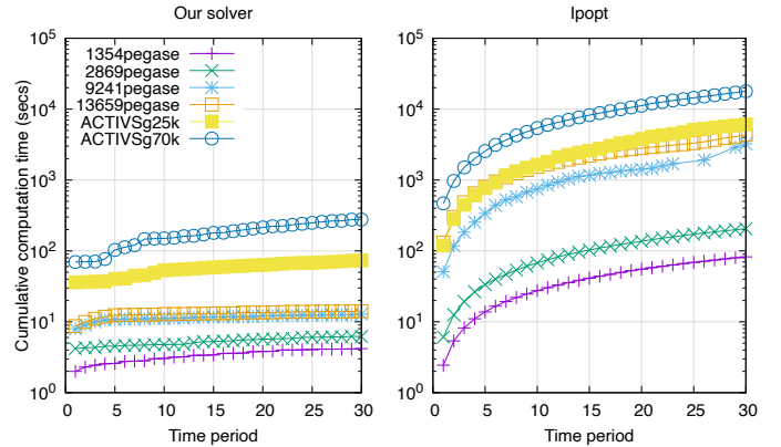
Figure 7: Cumulative computation time of warm start.
