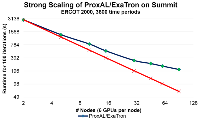
Figure 8: Scaling of ProxAL + ExaTron on Summit at OLCF
