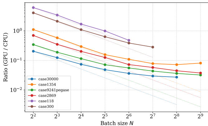
Figure 10: Parallel scaling of the total reduced Hessian accumulation \nabla^2 F with batch size N . A ratio value < 1 indicates a faster runtime compared with that of UMFPACK and AutoDiff on the CPU in absolute time. The dotted lines indicate the linear scaling reference. Lower values imply a higher computational intensity.
