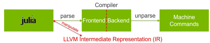
Figure 1: Julia’s just-in-time compilation enables LLVM IR manipulation through expression transformations.
