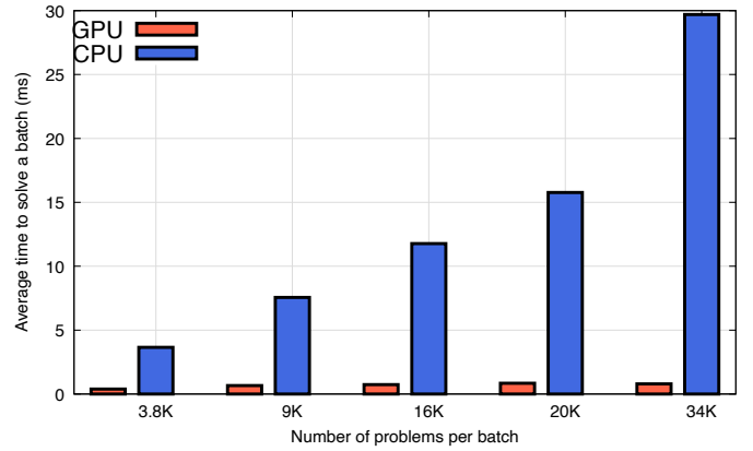
Figure 6: Performance comparison: 40 CPUs vs 6 GPUs on a Summit node. The GPUs solve batches of 34K problems 40 times faster than the CPUs do.
