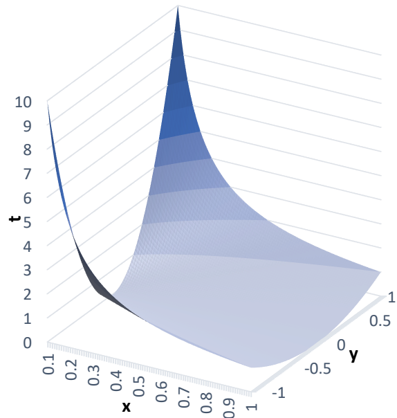
Figure 1: Graph of the perspective function t = y^2/x .
