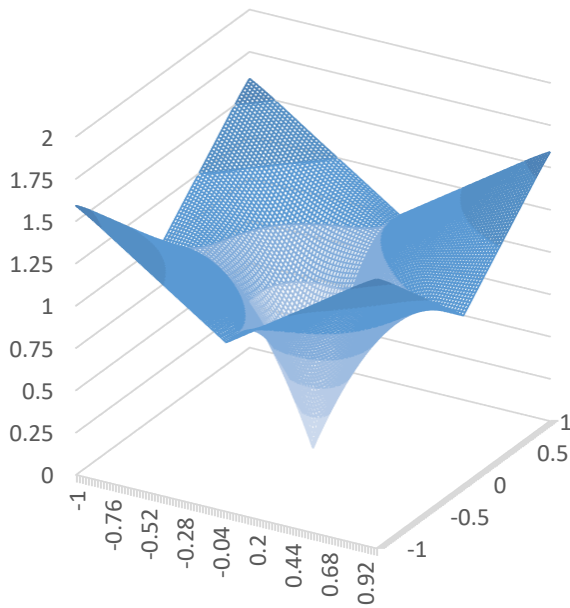
(b) Rank-one reformulation
