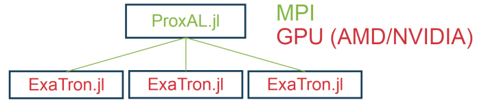
Figure 5: Two-stage parallelization strategy. ProxAL decomposes along the periods, and each ExaTron instance solves a single ACOPF.
